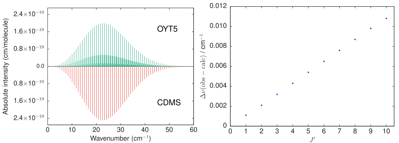
Figure 6. Comparison of the NaOH OYT5 line list with CDMS (Müller et al. 2001, 2005). The left-hand panel shows an OYT5 stick spectrum at T = 300 K plotted against all transition data from CDMS. The right-hand panel shows the residual errors \Delta\nu(\text{obs} - \text{calc}) (in \text{cm}^{-1} ) between the observed CDMS wavenumbers and the computed OYT5 wavenumbers up to J' = 10 , where J' is the rotational quantum number of the upper state involved in the pure rotational transition.
