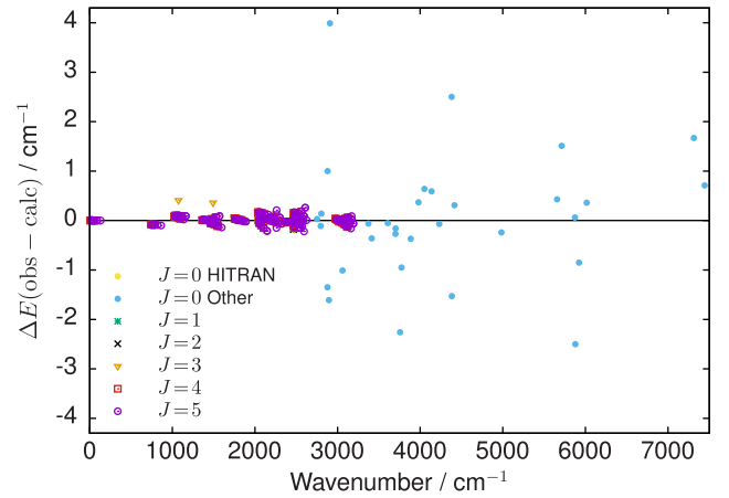
Figure 1. Fitting residuals, \Delta E(\text{obs-calc}) = E_{\text{obs}} - E_{\text{calc}} , of the 739 energy levels used in the PES refinement.
