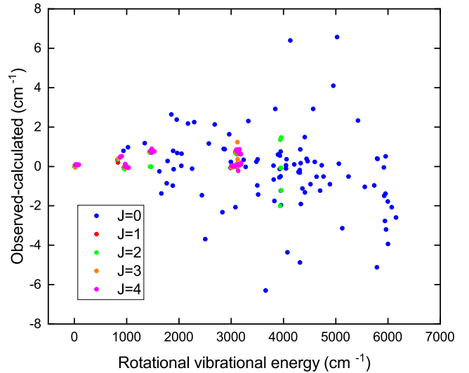
Figure 2. Observed–calculated rotational-vibrational energies after refinement. Vibrational energies (blue dots) with larger discrepancies were given a 1000 times smaller weighting in the refinement with respect to HITRAN vibrational energies.
