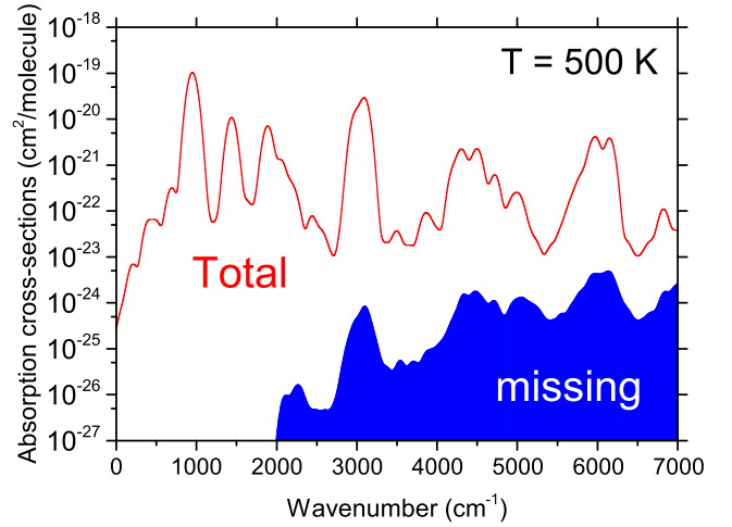
Figure 3. The vibrational cross-sections: total compared to the missing contribution due to the vibrational pruning.
