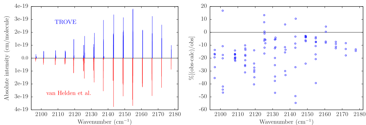
FIG. 2. Absolute line intensities of the \nu_3 band for transitions up to J = 16 (left) and the corresponding residuals ( \% \left[ \frac{\text{obs-calc}}{\text{obs}} \right] ) (right) when compared with measurements from van Helden et al. 89
