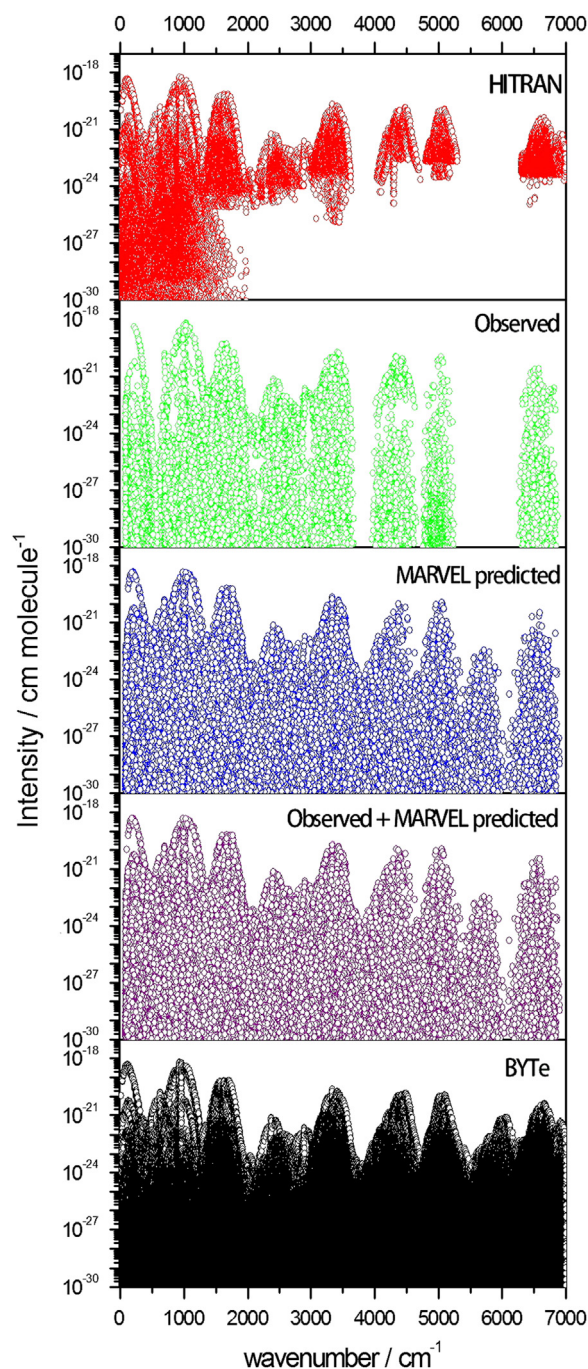
Fig. 2. Comparison of spectra at 296 K for one-photon absorption transitions of ^{14}\text{NH}_3 up to 7000\text{ cm}^{-1} . Top panel – lines present in the HITRAN [184] database; second panel – observed transitions present in MARVEL; third panel – MARVEL predicted transitions, omitting lines which have already been observed; fourth panel – sum of the observed and MARVEL predicted transitions; and bottom panel – all lines predicted by variational computations (BYTe [176]). Except for the top panel, all intensities come from BYTe.
