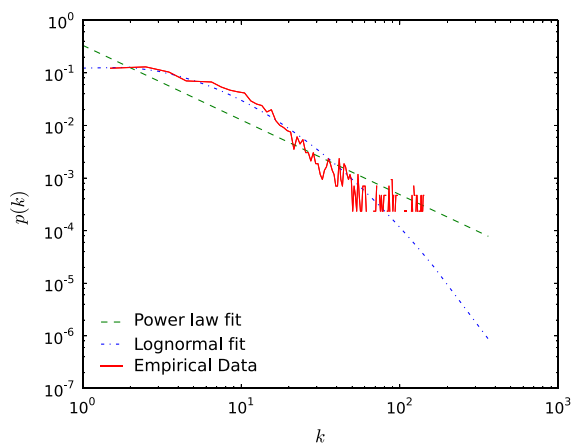
Fig. 1. Size-frequency distribution of the experimental spectroscopic network of ^{14}\text{NH}_3 .
