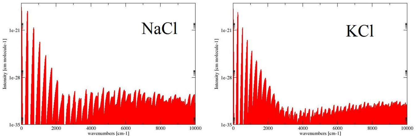
Figure 3. Absorption spectra of Na 35 Cl and 39 K 35 Cl at 300 K.
