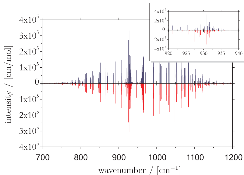
Figure 6. Absorption spectra of \text{NH}_3 at T = 300 K ( \text{cm mol}^{-1} ): BYTe versus HITRAN.
