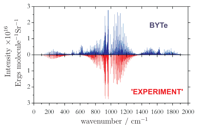
Figure 7. Emission spectra of \text{NH}_3 at T = 900 K ( \text{erg molecule}^{-1} \text{Sr}^{-1} ). The ‘experimental spectrum’ (lower display) is reconstructed using the Einstein coefficients from Yu et al. (2010).
