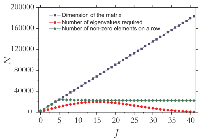
Figure 1. Dimensions of the E -symmetry matrices (squares), the corresponding number of eigenvalues below 18\,000\text{ cm}^{-1} (circles) and number of non-zero elements on each row (diamonds).
