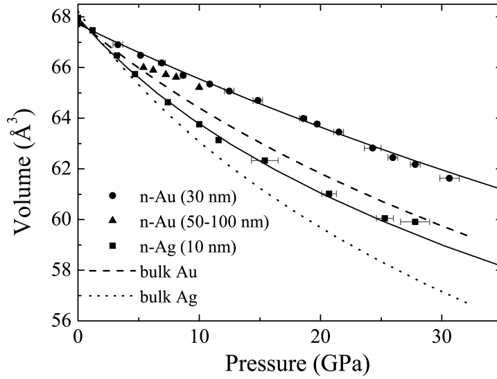
Fig. 2. Nano equation of state. Powder X-ray diffraction measurements of unit cell volume of nanocrystalline powders of Au and Ag as a function of pressure measured in a Diamond Anvil Cell. Reprinted (abstract/excerpt/figure) with permission from “Unexpected High Stiffness of Ag and Au Nanoparticles”, Q. F. Gu, G. Krauss, W. Steurer, F. Gramm, A. Cervellino, Phys. Rev. Lett. 100 045502 (2008). Copyright (2008) by the American Physical Society.
