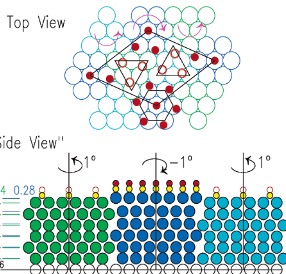
Figure 3. Structural model of the Pt(111) surface relaxation induced by the (\sqrt{19} \times \sqrt{19}) -13CO phase. Small solid and open circles represent the CO molecules in nearly top and bridge sites, respectively. Large circles in different colors represent the Pt atoms in three groups with different rotation centers. The “side view” is not a projection, but a simplified picture to illustrate schematically the grouping and layer expansion. The top layer expansions of 0.28 and 0.04 Å from the lattice positions are amplified 4-fold for visibility.
