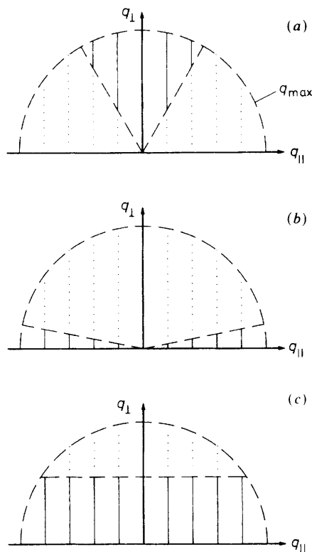
Fig. 3. Schematic reciprocal space diagrams showing the limited range of diffraction data available to different techniques. The rods represent data. The hemispherical diffraction limit is an arbitrary total resolution cut-off. (a) LEED: The cone angle is set by the angular size of the screen ( 120^\circ here). LEED system designs might vary slightly but will not affect this picture dramatically. (b) Four-circle X-ray diffraction 2 : Here the cone angle is given by the maximum tilt angle accessible to the sample, limited by feedthroughs etc. ( 11^\circ here 1 ). The same tilting limitations and diagram apply to transmission electron diffraction (TED). (c) Five-circle X-ray diffraction 3 or X-ray diffraction with out-of-plane detector arm 5,17 : The limiting perpendicular limit is given by the wavevector times the maximum inclination angle ( ca. 20^\circ ).
