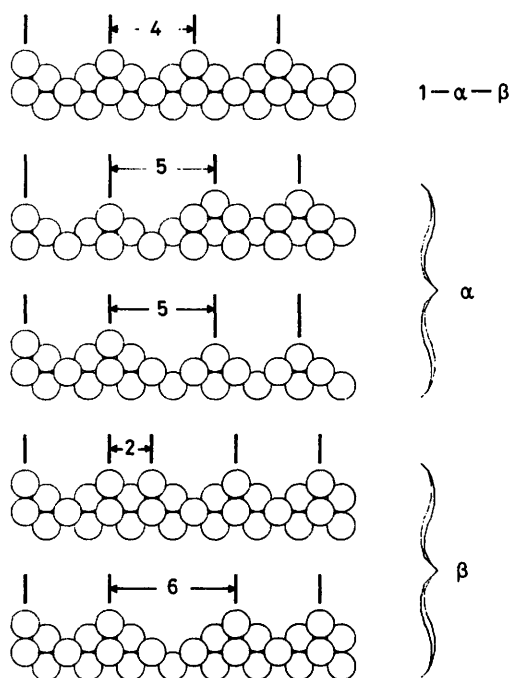
Fig. 5. Atomic models of Pt(110) surfaces containing a perfect 1 \times 2 reconstruction (top), the same interrupted by a single height step (middle), and the same interrupted by antiphase defects (bottom). The lateral phase shift across the defect is indicated in units of half a unit cell spacing. \alpha , \beta and 1 - \alpha - \beta refer to the assumed probabilities per site of the various configurations.
