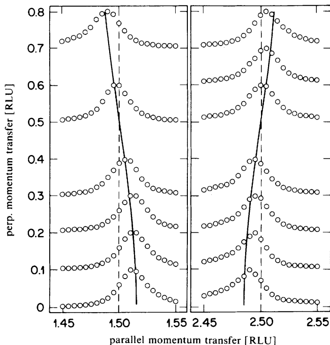
Fig. 4. Locus of the peak position in reciprocal space for a missing-row structure containing random steps, adapted from Fenter and Lu. 19 Superimposed on this are our data for Pt(110) on a normalised vertical scale, showing good agreement with the prior predictions.
