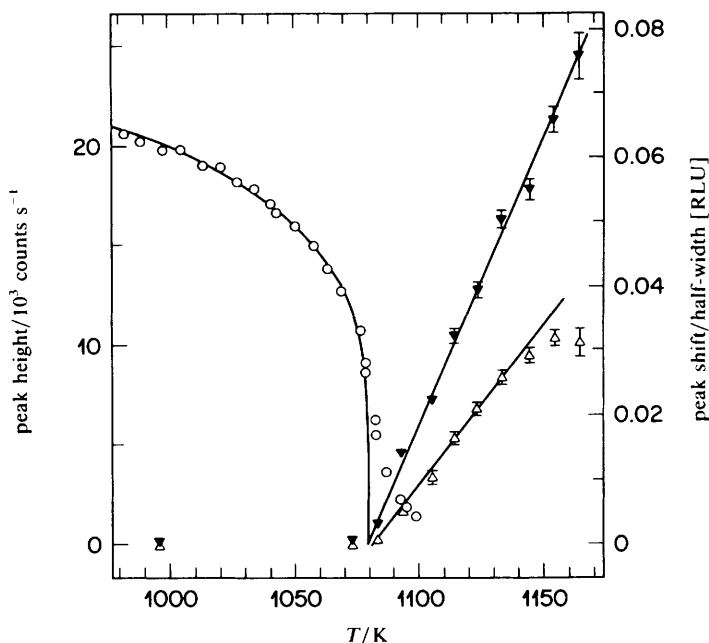
Fig. 6. Temperature dependence of the Lorentzian fitting parameters of the Pt(110) radial lineshape measured at (1.5, 0, 0.06). ○, peak height fit with T_c = 1080 K, \beta_c = 0.11 . ▼, Half-width; △, shift.
