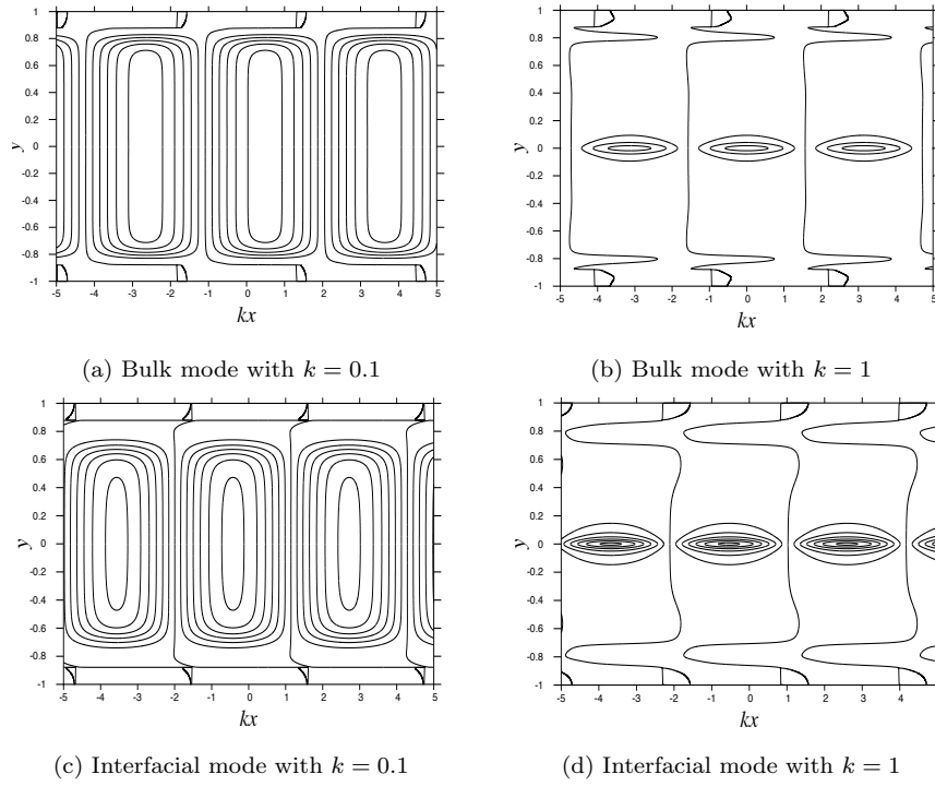
Figure 27: Streamlines of the perturbation flows for the unstable sinuous bulk and sinuous interfacial modes for different values of wavenumber k . The parameter values used are W = 2 , \Phi = 0.001 , \Lambda = 0.20 , \theta = 0.1 and \Gamma = 0.0192 . The interface location is \kappa = 0.8791 .
