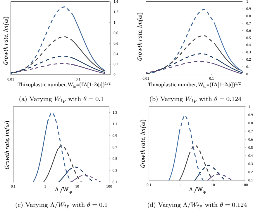
Figure 25: Figures (a) and (b): growth rate against thixoplastic number for bulk modes with shear-banding parameter variable fixed. Figures (c) and (d): growth rate plotted against material parameter \Lambda/W_{tp} with fixed \theta . For all plots: W = 2 , k = 0.1 and \Phi = 0.001 ; from top to bottom: \Lambda = 0.1, 0.2, 0.5 and 1 . Dashed lines represent base-states with a jump in the fluidity profile.
