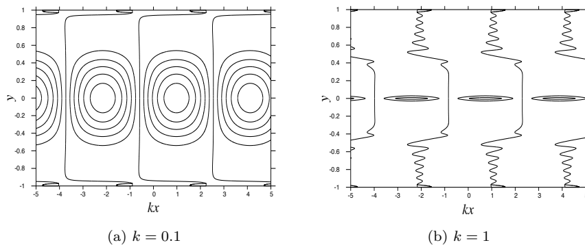
Figure 28: Streamlines of the perturbation flows for the unstable sinuous interfacial modes for different values of wavenumber k . The parameter values used are W = 2 , \Phi = 0.001 , \Lambda = 0.20 , \theta = 0.5 and \Gamma = 0.00032 . The interface location is \kappa = 0.9714 .
