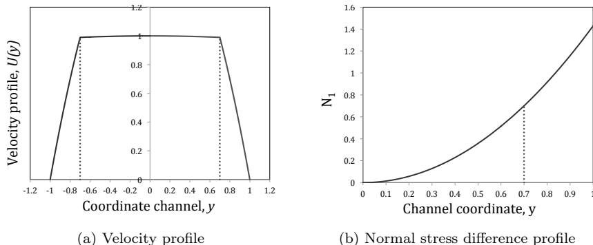
Figure 29: Velocity (a) and first normal stress difference (b) profiles for an Oldroyd-B fluid with concentration and Weissenberg number variable. The parameters used are: C_1 = 0.1 , C_2 = 100 , W_2 = 4 and \kappa = 0.7 (vertical dotted lines).
