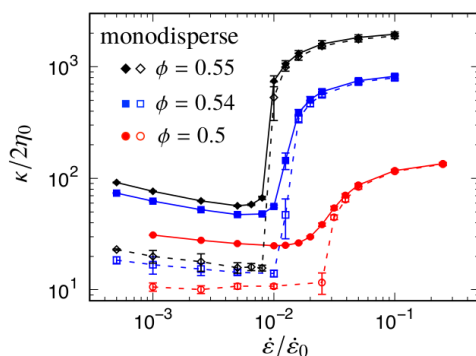
FIGURE 2. Plots of effective viscosity against flow rate for suspensions at different volume fractions. Solid symbols, solid lines: extensional flow; Open symbols, dashed lines: shear flow. Taken from Seto et al. (2017), figure 2.
