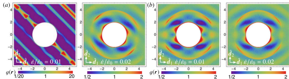
FIGURE 1. (a) The pair distribution function g(\mathbf{r}) below thickening (left) and above thickening (right) for simple shear flow of a monodisperse suspension. (b) The equivalent plots for planar extensional flow. Taken from Seto et al. (2017), figure 6.
