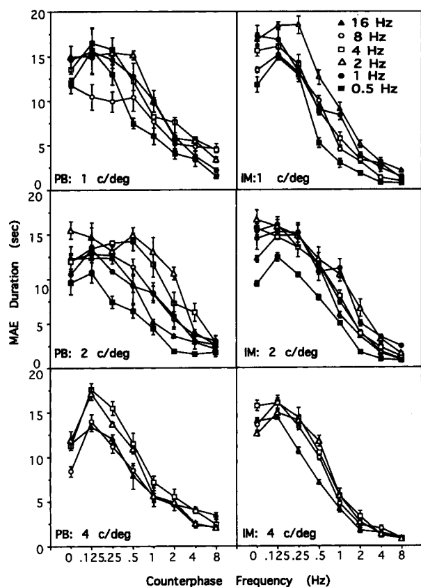
FIGURE 2. Magnitude of MAE as a function of the temporal frequency of the counterphasing test grating. The data for the two observers are shown in separate columns and the data for the three adapting spatial frequencies (as well as test spatial frequencies) are shown in separate rows. The temporal frequency of the adapting grating is shown in the caption and the temporal frequency of the adapting grating is shown in the legend. The spatial frequency of the test grating was the same as that of the adapting grating in each case. The temporal frequency of the test grating is shown on the x-axis with semi-log coordinates (to permit the inclusion of the 0 Hz data, where the test grating was static). The duration of the MAE is shown on the y-axis. Each data point is the mean of at least four observations. Error bars show \pm S.E.
