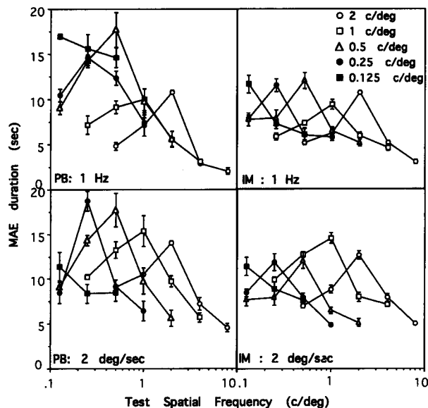
FIGURE 3. Magnitude of MAE as a function of the spatial frequency of the counterphasing test grating. The data for the two observers are shown in separate columns and the data for the separate temporal frequencies are shown in separate rows. The spatial frequency of the adapting grating is shown in the caption. In the top row, the temporal frequency of the adapting grating was 1 Hz (its speed varied), in the bottom row, the speed of the adapting grating was 2 deg/sec (its temporal frequency varied). The spatial frequency of the adapting grating is shown on the x-axis with semi-log coordinates. The temporal frequency of the test grating was 0.25 Hz in each case. The duration of the MAE is shown on the y-axis. Each data point is the mean of at least four observations. Error bars show \pm 1 S.E.
