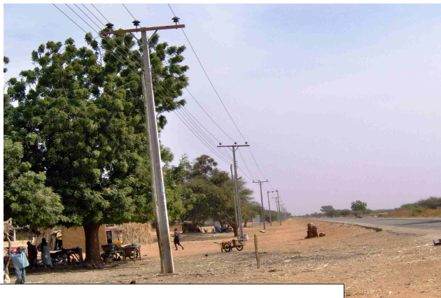
Stringing of overhead lines
