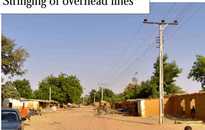
Stringing of overhead lines
