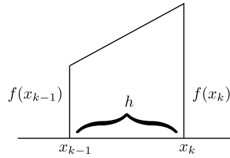
Figure 4.10: Trapezium constructed over each piece of the interval, where each piece has width h .
