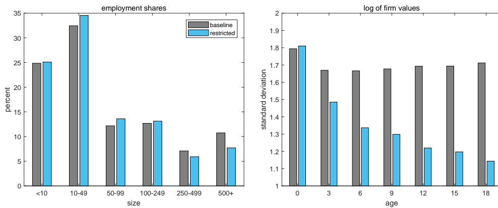
Figure 9. : Model comparison: baseline and restricted version
