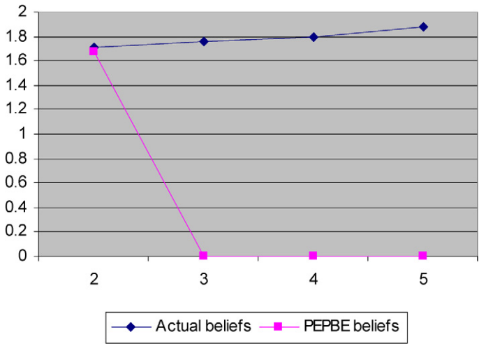
Fig. 1. PEPBE and observed average beliefs about the expected value of an investment, given a history that consists of successes only (Treatment A).
