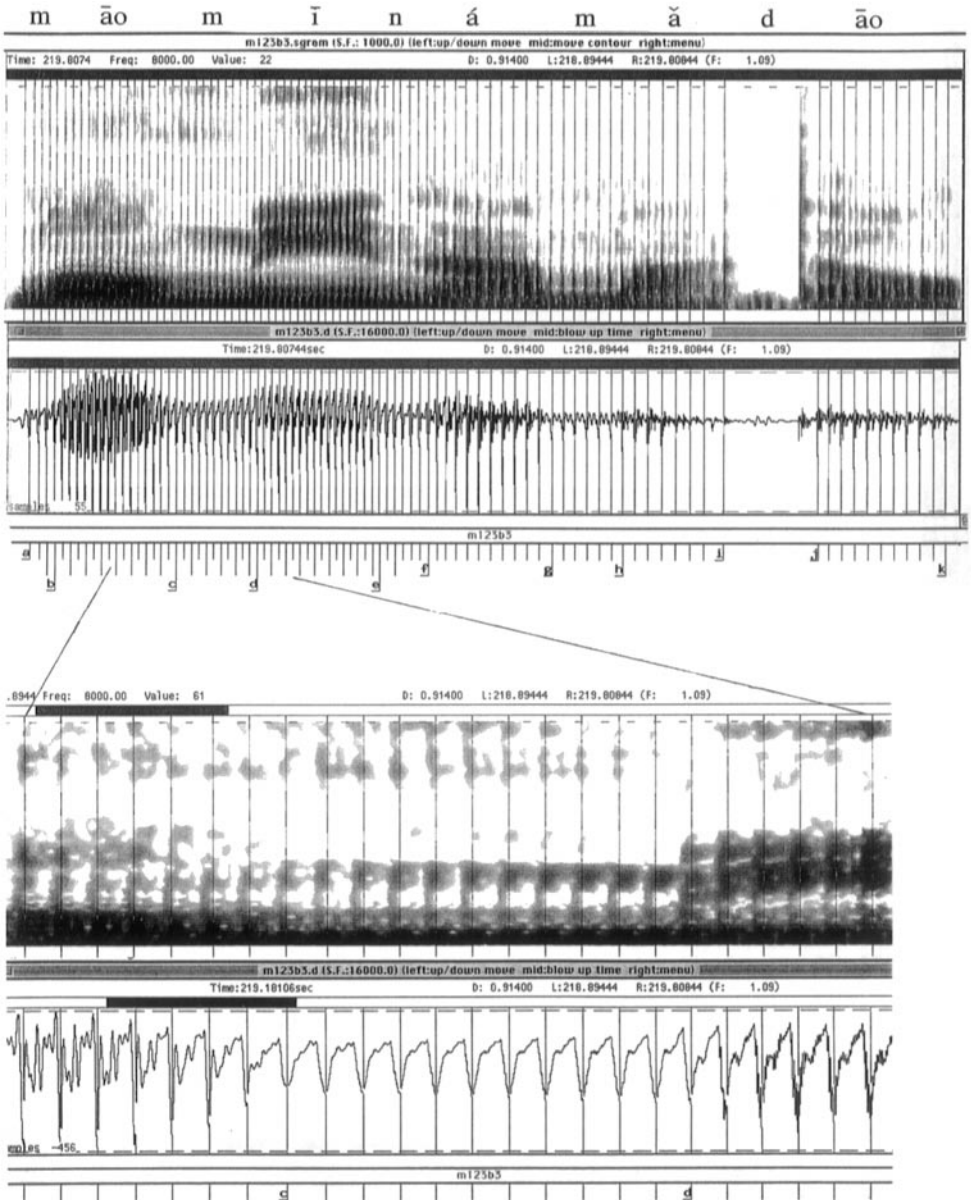
Figure 1. Top panel: an example of consonant and vowel segmentation and vocal-cycle marking. The vocal-cycle marking was produced by the “epochs” program in the ESPS package. The segmentation was done manually. A V–N boundary is located in the vocal pulse where the oral cavity is evidently closed; a N–V boundary is located in the vocal pulse where the oral cavity is evidently open. Evidence for the instants of oral cavity opening and closing could be found both in the spectrogram and in the waveform, as shown in the expanded view of the spectrogram and waveform in the bottom panel.
