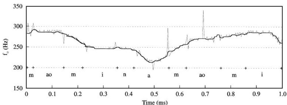
Figure 2. A raw f_0 curve obtained by taking the inverse of vocal periods (thin line), and the same curve after being smoothed by the trimming algorithm described in Appendix 1.
