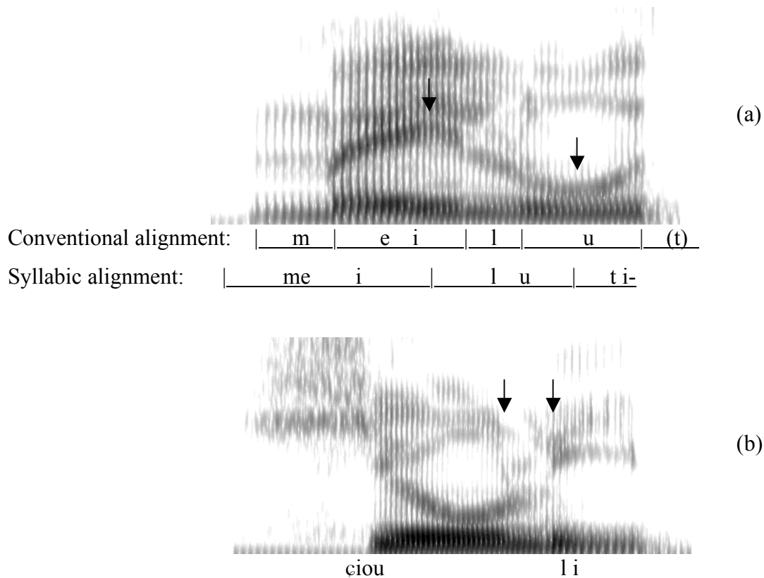
Figure 7. (a) Illustrative comparison of conventional alignment and proposed syllabic alignment. The entire utterance is [meiR luR (tienL χuoL)] (Light coal stove) in Mandarin (spoken by the first author), but only the spectrogram of meiR luR is displayed. The two arrows mark the onset and offset of the coproduced /u/. (b) Spectrogram of [ciouH liL (buF tʂouF)] (repair procedure) spoken by the first author. The two arrows mark the onset and offset of the /l/ murmur.
