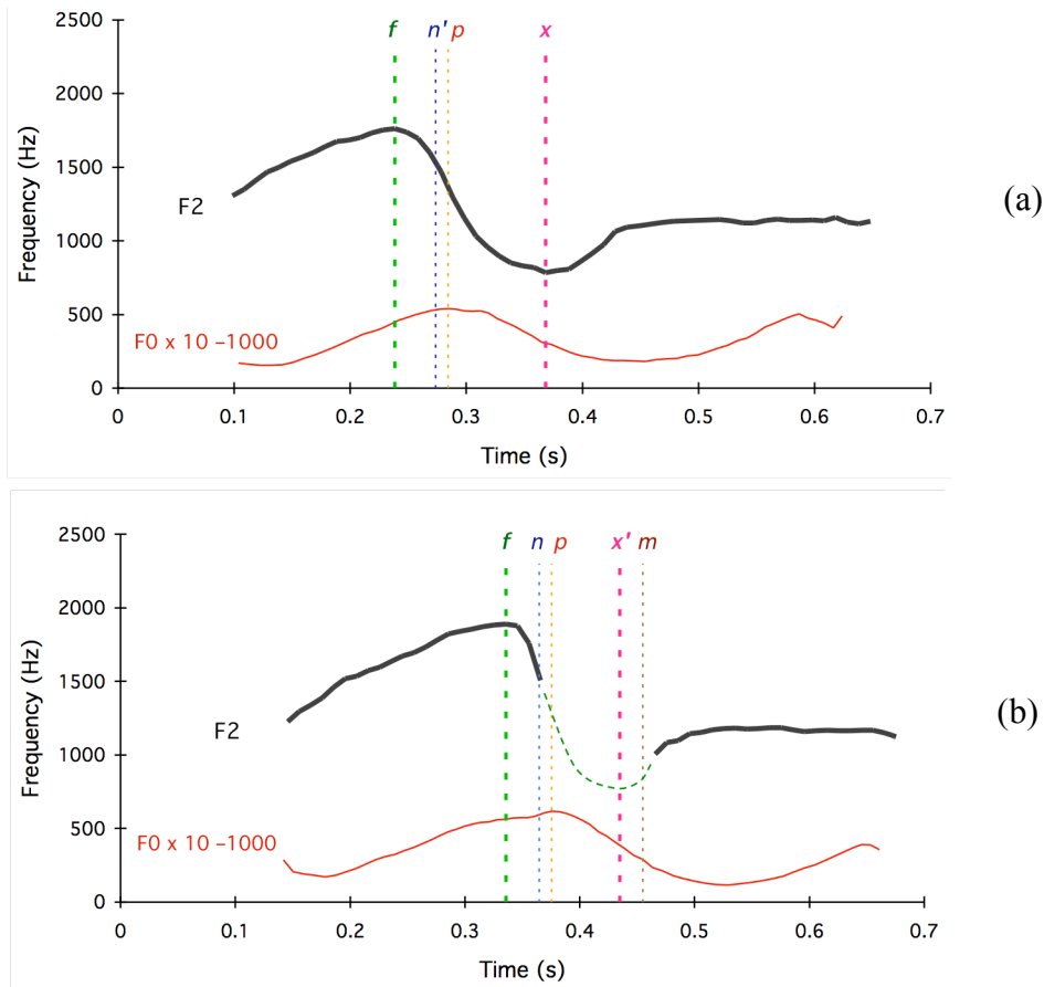
Figure 4. Schematic plots showing F2 and F 0 tracks of two Mandarin words uttered by a Mandarin speaker together with various alignment points. (a) [paɪR waR] (R = Rising tone). (b) [paɪR maR/].
