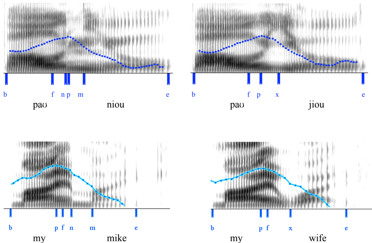
Figure 2. Illustration of markers placed in each word. Top: Mandarin nonsense words [paʊR niouL] (left) and [paʊR jiouL] (R and L stand for Rising and Low tone). The dotted lines are F 0 tracings generated by Praat. Bottom: English (General American): "MY mike" and "MY wife." (Capitalization indicates emphasis)
