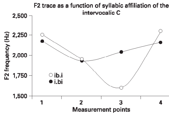
Figure 8. A plot of F2 measurements in /ib.i/ and /i.bi/ in Figure 4 of Lindblom et al. (2002), courtesy of Lindblom. See text for explanation.
