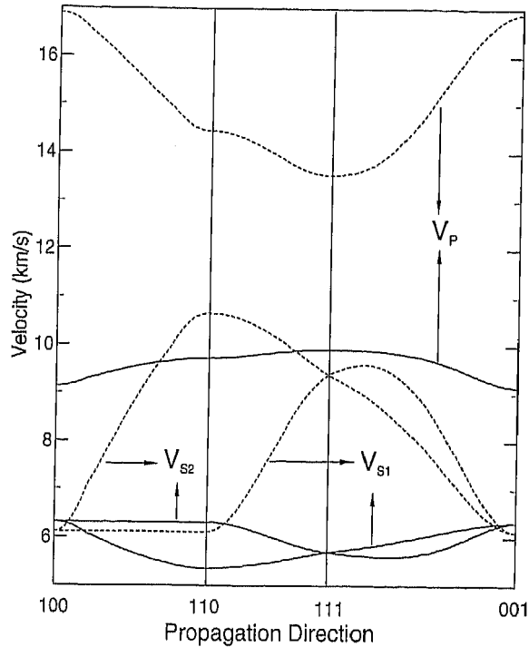
FIGURE 6. Dependence of the longitudinal ( V_p ) and two shear-wave velocities ( V_{s1} and V_{s2} ) of MgO on propagation direction at two pressures: the solid curves at 0 GPa and the dashed curves at 150 GPa.
