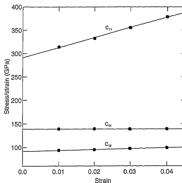
FIGURE 3. Stress/strain ratio vs. strain. The solid lines represent linear fits to the calculated values (solid circles) of stress/strain vs. strain for three elastic stiffness constants.
