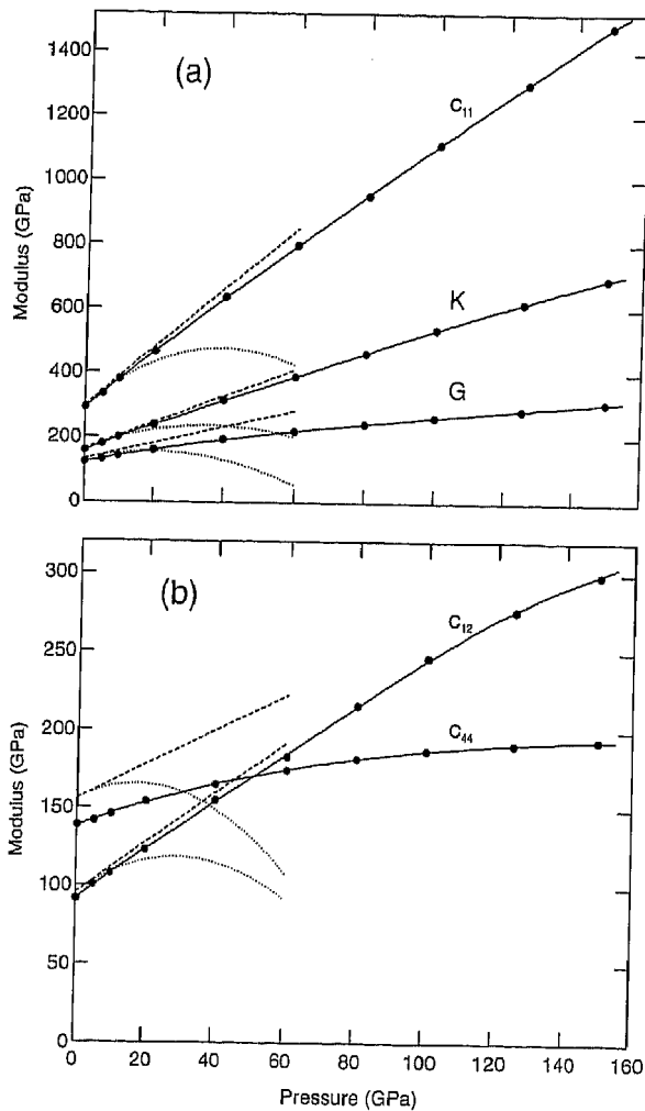
FIGURE 4. Pressure dependence of (a) c_{11} , K , and G , and (b) c_{12} and c_{44} of MgO. The symbols represent the calculated values, and the solid lines are the best fits. The first- and second-order extrapolations of low-pressure ultrasonic data (Jackson and Niesler 1982) to high pressure (up to 60 GPa) are shown by dashed and dotted lines, respectively.
