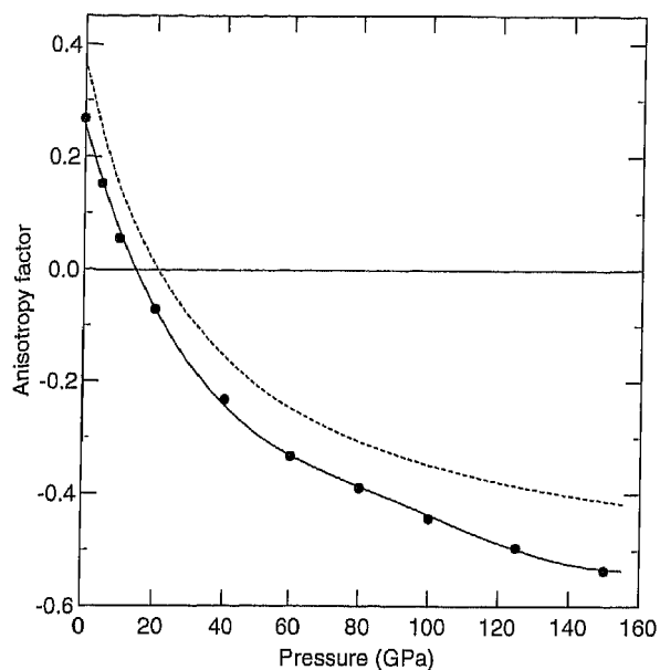
FIGURE 7. Pressure variation of the anisotropy factor, A , of MgO. The circles represent the calculated values. The first-order extrapolation from ultrasonic data (Jackson and Niesler 1982) is shown by the dashed line.
