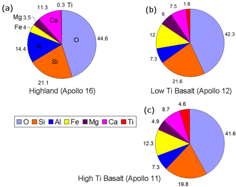
Figure 3. Example chemical compositions of lunar soils: (a) lunar highland minerals (Apollo 16); (b) low-Ti basalts (Apollo 12); and (c) high-Ti basalts (Apollo 11). Based on data collated by Stoesser et al. (2010) and reprinted from Planetary and Space Science , Vol. 74, Schwandt C, Hamilton JA, Fray DJ et al., 'The production of oxygen and metal from lunar regolith', pp.49–56, Copyright (2012), with permission from Elsevier.
