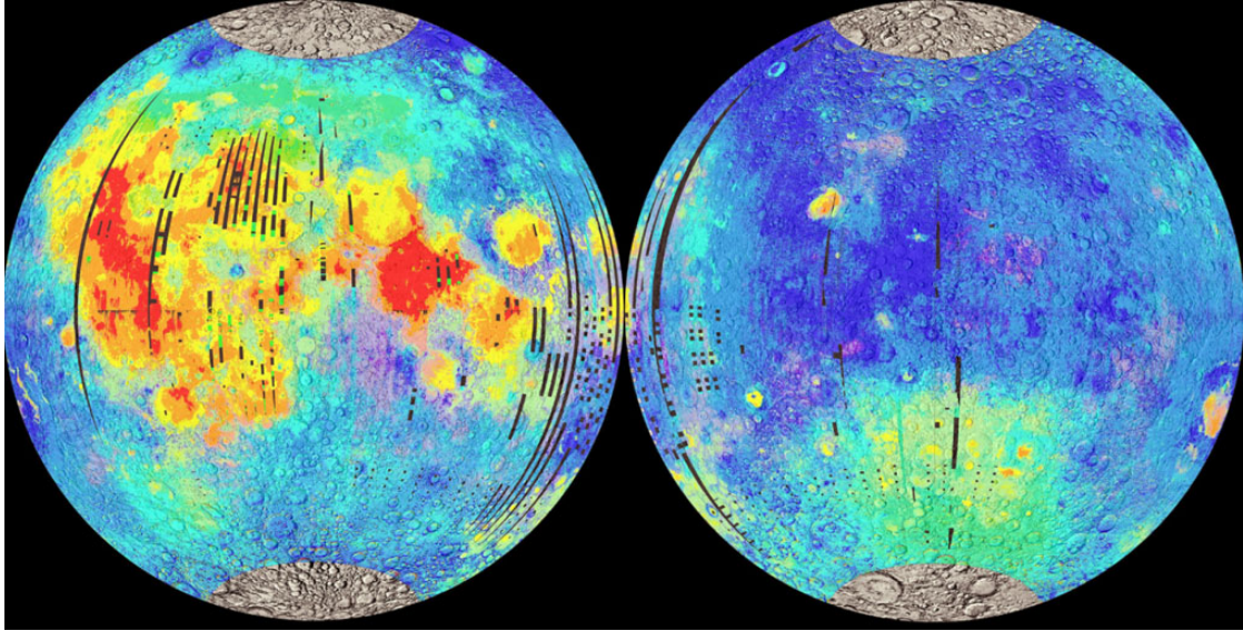
Figure 2. Distribution of regolith compositions on the lunar nearside (left) and the farside (right) based on Clementine multi-spectral imaging data. Blue: anorthositic highlands; yellow: low-Ti basalts; red: high-Ti basalts. The large yellow/greenish area in the southern hemisphere of the farside is the South Pole-Aitken Basin, where the colours mostly reflect the more Fe-rich nature of the lower crust exposed by the basin rather than basaltic material (Spudis et al., 2002; courtesy Dr Paul Spudis/LPI).
