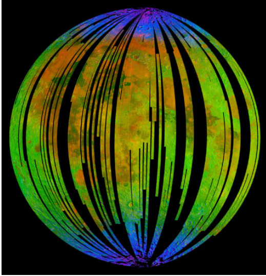
Figure 7. False colour image of the lunar nearside based on data obtained by the Moon Mineralogy Mapper ( M^3 ) instrument on India's Chandrayaan-1 mission. Blue represents areas where a 2.8 to 3.0 \mu\text{m} absorption band attributed to bound \text{H}_2\text{O}/\text{OH} was detected; red represents areas where the 1 \mu\text{m} band of the mineral pyroxene is strong, and picks out the basaltic maria; and green represents albedo. Note that evidence for hydration is restricted to high latitudes, but is much more extensive than areas of permanent shadow at the poles (image courtesy, NASA/ISRO/Brown University/R. N. Clark, USGS/AAAS).
