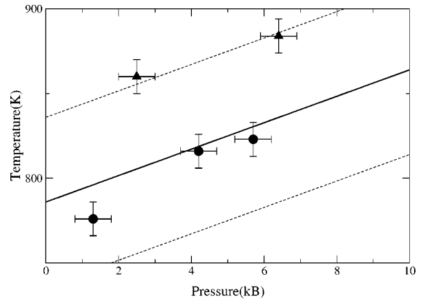
FIG. 4. Temperatures and pressures at which liquid and solid coexist in simulations containing 1000 atoms (circles) and 512 atoms (triangles). The solid line is the lower end of the melting curve calculated using the free-energy approach in Ref. 19 (see text), light dashed lines represent error bars.
