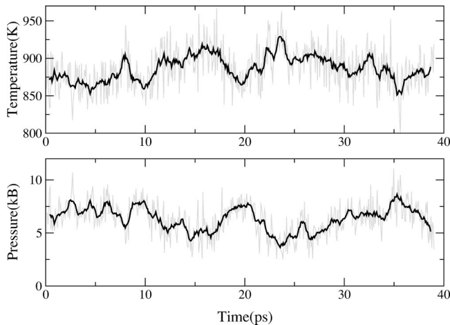
FIG. 3. Time variation of temperature (upper panel) and pressure (lower panel) during a simulation of solid and liquid Al in coexistence for a system containing 512 atoms. Gray lines—actual data; black lines—running averages over a 0.75 ps period.
