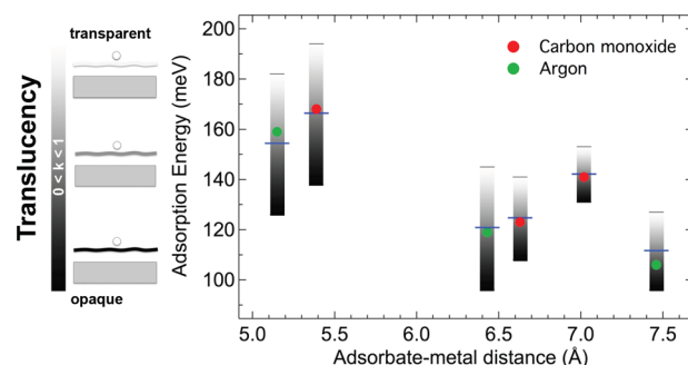
Figure 5. Adsorption energy dependence on adsorbate–metal distance for carbon monoxide molecules (red) and argon atoms (green) in the different configurations discussed in Figure 4, i.e. , on flat Gr and on the hills and valleys of corrugated Gr. Blue ticks indicate the results of best fit using the equation I = G + kS , where k is the factor accounting for the screening of the vdW interactions by Gr. Vertical bars correspond to the values of complete blocking (black region) and total transparency (white region) of Gr.
