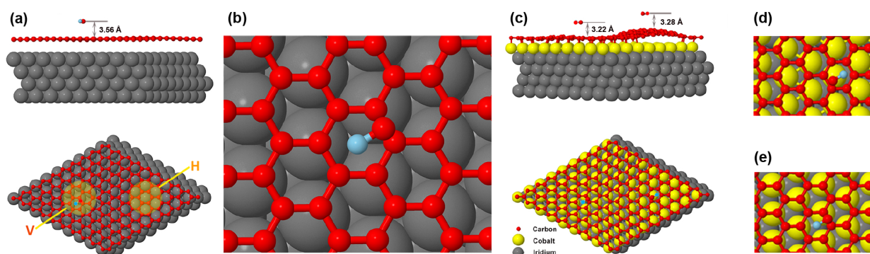
Figure 3. (a) Side and top views of the of the most stable CO adsorption configuration as found in our calculations. Gray atoms represent the Ir(111) surface; carbon atoms are displayed in red, and the oxygen atom is shown in blue. Valley and Hill regions are colored in the top view. (b) Local configuration of the CO molecule, with the O atom sitting above the center of a Gr hexagon and the C atom located in a bridge site. (c) Top and side views of the minimum energy CO adsorption configurations on the hill and valley of the Gr moiré unit cell on Co/Ir(111). Cobalt atoms are shown in yellow. (d, e) Local configuration of the adsorption configuration of CO in both valley (d) and hill (e) regions on Gr/Co/Ir(111).
