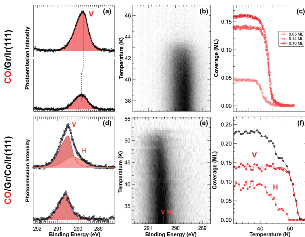
Figure 1. CO desorption from Gr/Ir(111). (a) C 1s spectra corresponding to different CO initial coverages ( \theta_{\text{CO}} = 0.08 ML (bottom) and 0.30 ML (top)), measured prior to the temperature ramp. (b) TP-XPS C 1s core level spectra showing its evolution during thermal desorption of CO from Gr/Ir(111). (c) Comparison of CO coverage evolution as a function of temperature for selected CO initial coverages. CO desorption from Gr/Co/Ir(111) (d) Selected spectra of the uptake corresponding to a coverage of 0.08 ML (bottom) and to saturation (top). (e) TP-XPS spectra acquired during a linear temperature ramp (the photoemission intensity is in gray scale) and (f) temperature evolution of V (valley) and H (hills) C 1s photoemission components of a 0.23 ML CO dose as a function of temperature.
