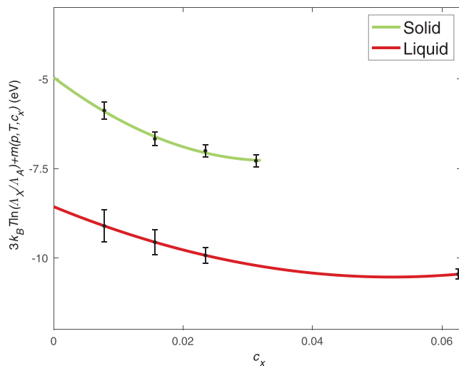
Figure 5. The calculated left-hand side of equation (14) (3k_B T \ln(\frac{\Delta x}{\Delta A}) + m(p, T, c_X)) shown as dots with the error bar. The curves are fits (corresponding to the right-hand side of equation (14)). Fitting parameters are listed in Table 1.
