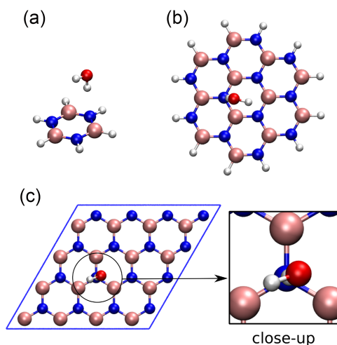
FIG. 1. (a) Water adsorbed on borazine ( \text{B}_3\text{N}_3\text{H}_6 ). (b) Water adsorbed on boronene ( \text{B}_{12}\text{N}_{12}\text{H}_{12} ). (c) Water adsorbed on a (4 \times 4) unit cell of a h-BN sheet with a close-up of the physisorption site. White spheres are hydrogen, red spheres are oxygen, pink spheres are boron, and blue spheres are nitrogen.
