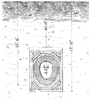
SECTION OF SEWER IN TUNNEL UNDER HORSE GUARDS.
