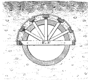
SECTION OF SEWER IN TUNNEL UNDER NEW RIVER EMBANKMENT.
