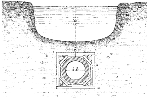
SECTION OF SEWER IN TUNNEL UNDER REGENT'S CANAL, CALEDONIAN ROAD.
