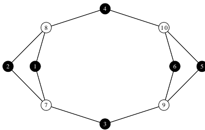
FIG. 1: An \alpha -Kuramoto partition with two parts.
