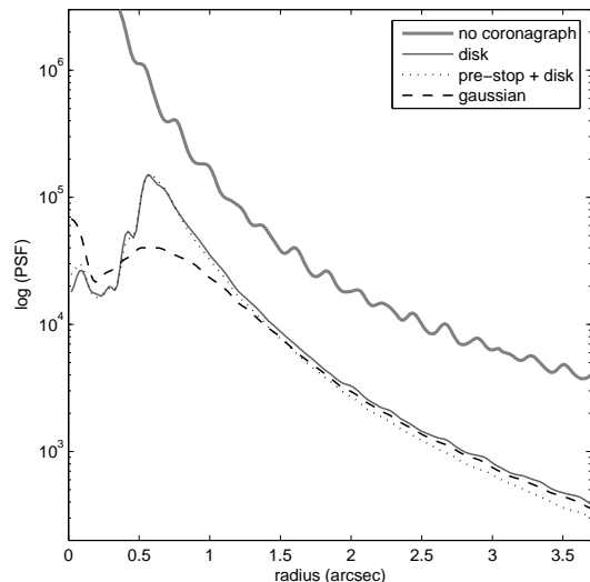
Figure 6. Simulated PSF profiles for the different shaped coronagraphic focal masks, the standard (80,20) Lyot stop was used for each. Characteristic width for each mask is 1.0 arcsec. Phase-screens corrected with a NAOMI-like simulated system - 2000, 256 \times 256 phase-screens with an 4 times FFT padding factor. Peak for no-coronagraph lies at 7 \times 10^8 .
