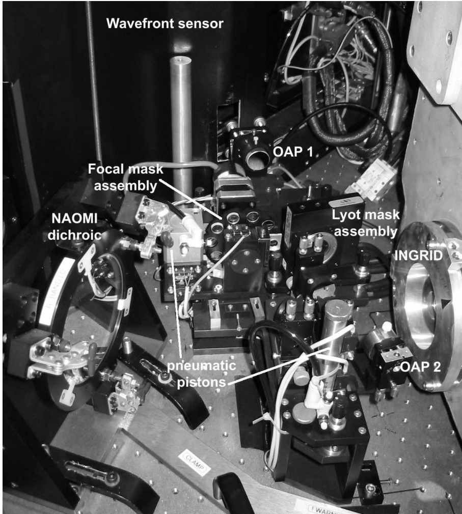
Figure 1. OSCA installed at the GRound based Adaptive optics Controlled Environment (GRACE) at the William Herschel Telescope. The light from NAOMI enters from the left through the dichroic and exits to the INGRID detector shown at the right-hand side of the picture. For scale, the hole spacing on the optical table is 25mm.
