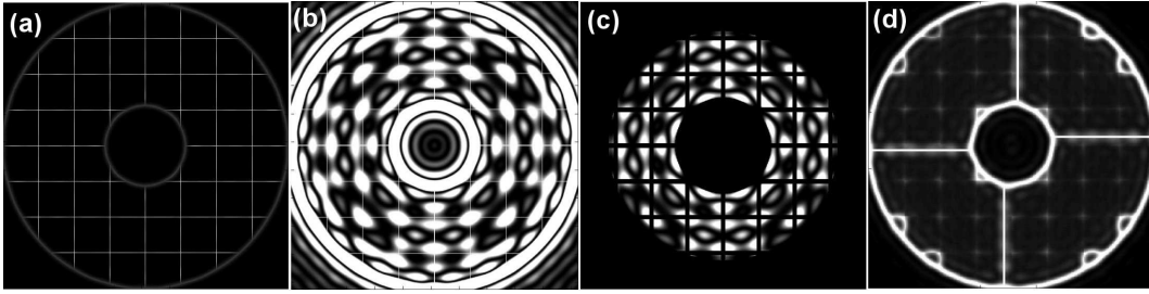
Figure 9. Pupil plane images after the application of a 2.0 arcsec hard circular stop. (a) aperture with segment gap representation of 2 pixels, image has been scaled to minimum and maximum levels; (b) same image as (a) but cut at a low intensity level to bring out faint structures; (c) as in (b) but with the grid-type Lyot mask applied; (d) no gaps, but full AO simulation showing the effect of phase errors between the segments, the secondary vane pattern based on the WHT aperture is included. The outer 4 and inner 4 segments are turned off in the AO simulation, the increased intensity about these indicates the greater phase mismatching. The simulation matches the mid-point of the segments in piston and so the corners are also at higher intensity due to phase errors.
