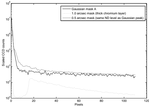
Figure 10. Results of lab testing of focal masks in an ideal coronagraphic system.
