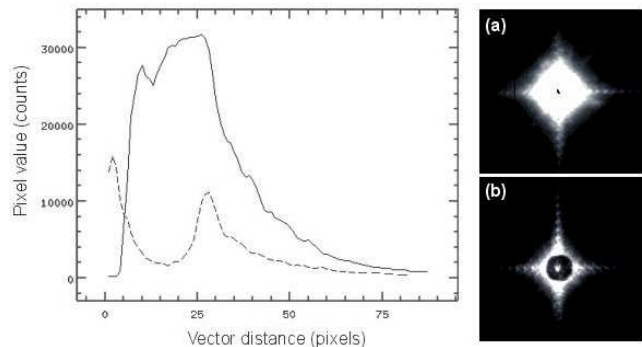
Figure 13. Cross-sections taken in the high-contrast ( 45^\circ ) direction from H -band images (a) without OSCA (solid line) and (b) with 2.0 arcsec mask (dashed line). The peak at zero is due to the OSCA mask having a small throughput. The jagged drop to zero ( < 25 pixels) with no coronagraph is due to detector saturation. The INGRID pixel scale is 0.04 arcsec/pixel.
