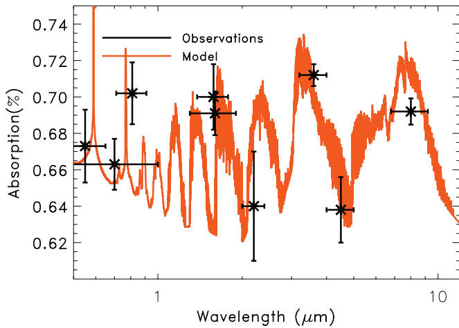
Figure 3. Simulated transmission spectrum of the transiting Hot Neptune GJ436b including the contribution of \text{CH}_4 , \text{H}_2 , and alkali metals in the wavelength range 0.5–9 \mu\text{m} . The simulation is a good fit to the observations with Spitzer -IRAC at 3.6, 4.5, and 8 \mu\text{m} , together with data collected by EPOXI in the range 0.5–1.0 \mu\text{m} (Ballard et al. 2010), HST NICMOS in the range 1.2–1.8 \mu\text{m} (Pont et al. 2009), and ground-based H band (Alonso et al. 2008) and K band (Cáceres et al. 2009).
