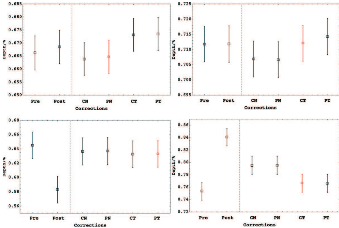
Figure A2. Measured transit depths at 3.6\ \mu\text{m} epoch 1 and 2 (left and right upper panels) and at 4.5\ \mu\text{m} (left and right lower panels), respectively, using the different families of corrections mentioned in the text. For each family, we only show the polynomial order which yielded the lowest BIC. The family which yielded the overall lowest BIC is plotted with a circle. “Pre” and “Post” are corrections using this same corrective function, but using only the pre-transit/post-transit data, respectively. (A color version of this figure is available in the online journal.)
