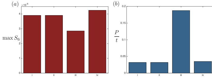
Fig. 11 (a) The maximum level of malonic semialdehyde in the system, (b) the eventual rate of 3HP production, both in the continuous replenishment of pyruvate case. In (b), we use P/t as the label for the y-axis as the levels of 3HP linearly increase with time (this continuous production is due to the continuous replenishment of pyruvate), and thus the appropriate measure here is the long-time production rate of 3HP. In both figures, the labels on the x-axis denote (i) Reference value (using the initial enzyme concentrations a_1 = a_2 = a_3 = a_4 = 1 ), (ii) Over-expressing PAND ( a_1 = 10, a_2 = a_3 = a_4 = 1 ), (iii) Concurrently over-expressing BAPAT and HPDH ( a_1 = a_4 = 1, a_2 = a_3 = 10 ), (iv) Over-expressing ALT ( a_1 = a_2 = a_3 = 1, a_4 = 10 ). The units of the y-axis are mM.
