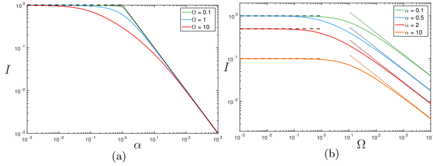
Fig. 4 The function I(\alpha, \Omega) defined in (12b). (a) Constant \Omega and varying \alpha . (b) Constant \alpha and varying \Omega . The solid curves are the numerically derived values, and the dashed and dotted curves are the asymptotic approximations for the small and large varying parameter, respectively. These approximations are defined in the text immediately below (12).
