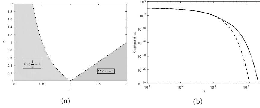
Fig. 12 (a) The shaded areas denote the regions in which there is switching of asymptotic orders in the long-time solution for limited initial pyruvate. In the region where \Omega < 1/\alpha - 1 , solutions (B2) hold. In the region where \Omega < \alpha - 1 , solutions (B4) hold. (b) Results for S_3 , taking \bar{k}_i = a_j = 1 for all i, j , and \alpha = 0.5 , thus falling into the region where \alpha < 1 and \Omega < 1/\alpha - 1 . The solid grey curve shows the numerical result, the dashed black curve shows the O(1) term in (B2a), and the dotted black curve shows the full expression given in (B2a). The latter two asymptotic results show excellent agreement with the numerical result until t \approx 10^3 , where asymptotic switching occurs, and the O(\varepsilon) term in (B2a) dominates.
