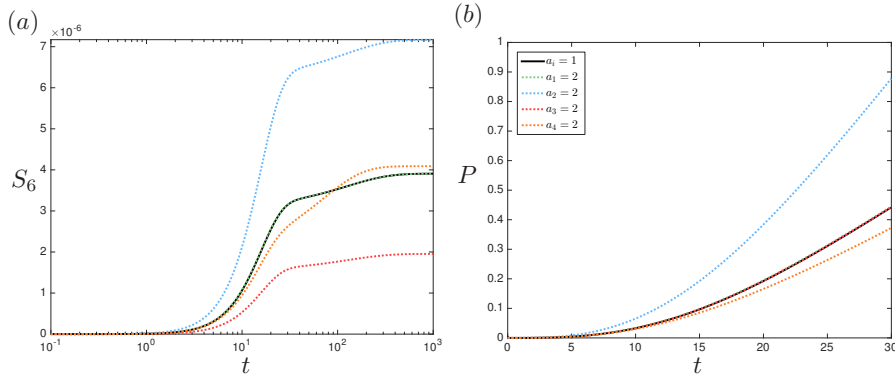
Fig. 7 Numerical solutions in the continuously replenished pyruvate case for the dynamic concentrations of (a) malonic semialdehyde and (b) 3HP. We use the parameter values given in table 2 for all simulations, and initial dimensionless enzyme concentrations of 1 unless specified in the legend. The solid black line corresponds to the reference simulation where a_i = 1 for i = 1, 2, 3, 4 .
