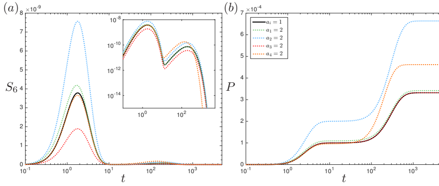
Fig. 2 Numerical solutions in the non-replenished pyruvate case for the dynamic concentrations of (a) malonic semialdehyde and (b) 3HP. We use the parameter values given in table 2 for all simulations, and initial dimensionless enzyme concentrations of 1 unless specified in the legend. The solid black line corresponds to the reference simulation where a_i = 1 for i = 1, 2, 3, 4 .
