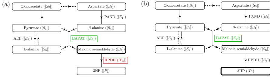
Fig. 9 A schematic to highlight the effect of over-expressing a given enzyme in the continuous replenishment case on (a) malonic semialdehyde and (b) 3HP. The underlying network and the arrows between the nodes are explained in figure 1. An enzyme that is boxed and red/green means that over-expressing this enzyme causes a/an decrease/increase in the metabolite of interest. Our goal is to reduce the levels of malonic semialdehyde whilst increasing the levels of 3HP, where possible.
