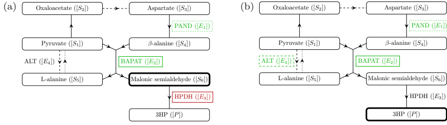
Fig. 6 A schematic to highlight the effect of over-expressing a given enzyme in the no replenishment case on (a) malonic semialdehyde and (b) 3HP. The underlying network and the arrows between the nodes are explained in figure 1. An enzyme that is boxed and red/green means that over-expressing this enzyme causes a/an decrease/increase in the metabolite of interest. Our goal is to reduce the levels of malonic semialdehyde whilst increasing the levels of 3HP, where possible. A dashed box denotes that the over-expression has diminishing returns with no upper bound, and a dotted box denotes that the over-expression has diminishing returns with an upper bound.
