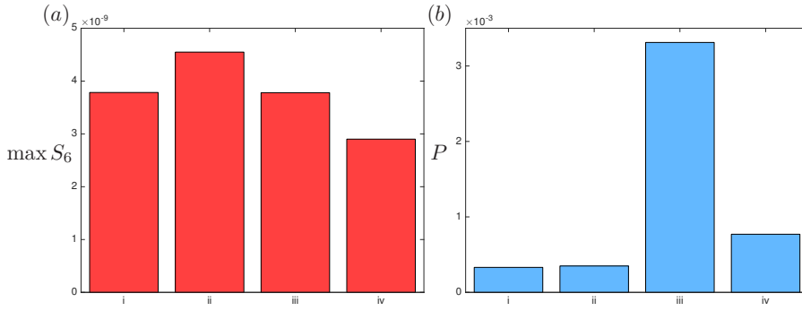
Fig. 10 (a) The maximum level of malonic semialdehyde in the system, (b) the total 3HP produced, both in the no replenishment of pyruvate case. In both figures, the labels on the x-axis denote (i) Reference value (using the initial enzyme concentrations a_1 = a_2 = a_3 = a_4 = 1 ). (ii) Over-expressing PAND ( a_1 = 10 , a_2 = a_3 = a_4 = 1 ), (iii) Concurrently over-expressing BAPAT and HPDH ( a_1 = a_4 = 1 , a_2 = a_3 = 10 ), (iv) Over-expressing ALT ( a_1 = a_2 = a_3 = 1 , a_4 = 10 ). The units of the y-axis are mM.
