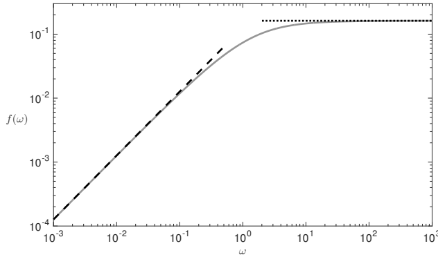
Fig. 5 The function f(\omega; u(\omega)) defined in (13) is given by the grey curve. The dashed and dotted black curves are the small and large \omega approximations, respectively. These approximations are defined in the text immediately below (13).
