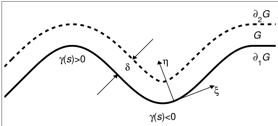
FIG. 1. Domain G and curvilinear coordinates \xi, \eta . The solid line denotes the boundary \partial_1 G with the Dirichlet boundary condition, and the dotted line — the boundary \partial_2 G with the Neumann boundary condition.
