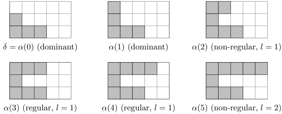
Figure 5: Cases arising for \alpha(i) in proof of Lemma A.23.
