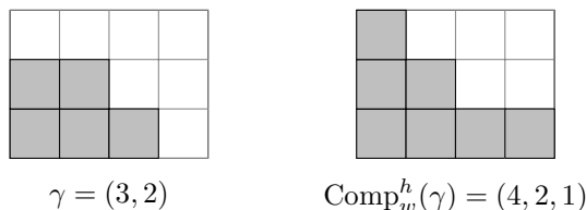
Figure 3: Young diagram \gamma = (3, 2) and its complement for h = 3, w = 4 .
