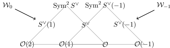
Figure 2: Windows used in calculation of window-shift \omega_{-1,0} for Grassmannian example r = 2, d = 4 .
