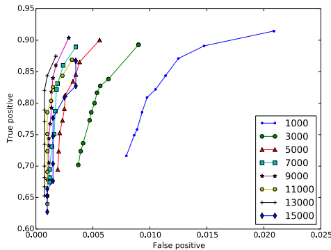
Figure 16: Attack accuracy for 17,000 unmonitored web pages. Each line represents a different number of unmonitored web pages that were trained, while varying k , the number of fingerprints used for classification.
