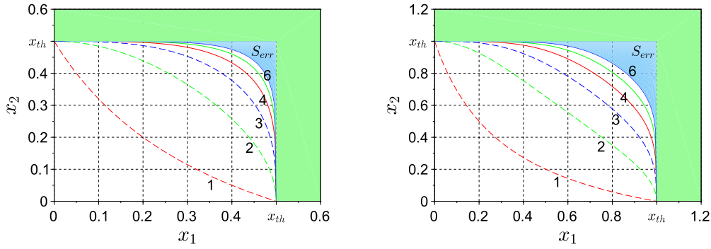
Fig. 3. Lines — the boundary separating the gene classifier responses according to Eq. (17), corresponding to \hat{p} = (\hat{1}, \hat{1}) , for the integer values of the cooperativity coefficient m = 1, 6 (indicated next to the curves; the unlabeled curve is for m = 5 ), with x_{th} = 0.5 (left panel) and x_{th} = 1.0 (right panel). Pale green area — region of the positive responses of the Boolean classifier (6), same as in panel (C) of Fig. 1, which is to be approximated by the gene circuit. Pale blue area S_{err} — region of false positive responses of the gene classifier for m = 6 . Notice that higher cooperativity m brings the classification boundary closer to the desired boundary, and choosing the threshold value x_{th} = 0.5 leads to a slight improvement over x_{th} = 1.0 . (For interpretation of the references to colour in this figure legend, the reader is referred to the web version of this article.)
