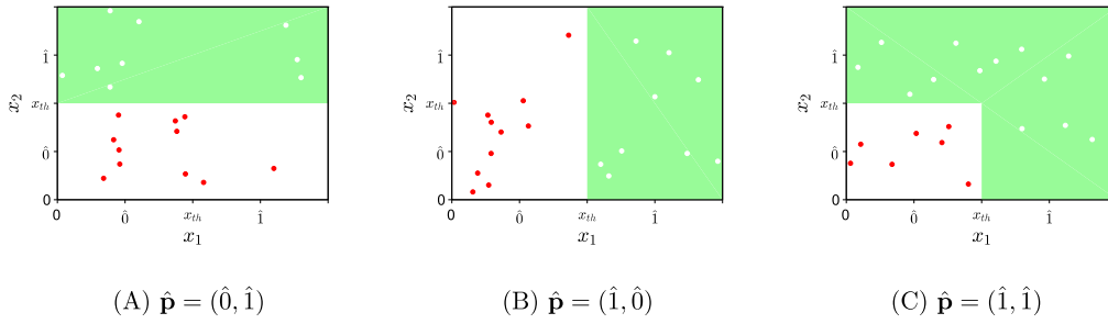
Fig. 1. Output of the classifier defined by Eqs. (6), (7) as a function of the continuous inputs x_1, x_2 (white area — \widehat{Out} = \hat{0} , pale green area — \widehat{Out} = \hat{1} ) for the 3 variants of the Boolean parameter vector \hat{\mathbf{p}} , as indicated. Threshold x_{th} separates the regions corresponding to Boolean \hat{0} and \hat{1} along the axes. Examples of valid training sets which uniquely identify each variant are shown as scatter plots with filled circles (red — \widehat{Out}^{(i)} = \hat{0} , white — \widehat{Out}^{(i)} = \hat{1} ). Notice that the training set in each panel does not match the classification rules in the other panels. (For interpretation of the references to colour in this figure legend, the reader is referred to the web version of this article.)
