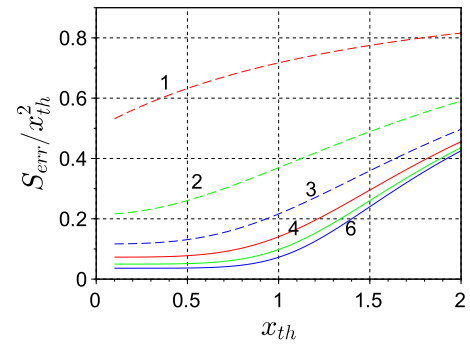
Fig. 4. Classification error measure S_{err}/x_{th}^2 (characterizing the accuracy to which the gene classifier approximates the Boolean model (6)) as a function of the threshold x_{th} for the integer values of the cooperativity coefficient m = 1, 6 (indicated next to the curves; the unlabeled curve is for m = 5 ). Notice that higher cooperativity m and lower threshold x_{th} improve the accuracy.
