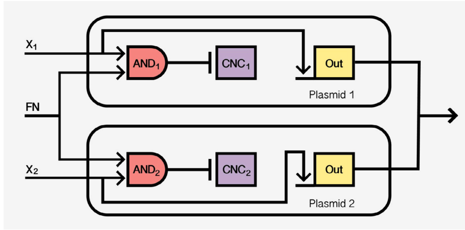
Fig. 2. Scheme of the gene network implementing the learnable Boolean classifier described in Section 3. The network is composed of two parts located on separate plasmids. The network inputs are x_1, x_2 — the classifier inputs, and FN (“Forced Negative”) — the logical negation of the correct answer used in the learning mode only. Output is encoded by the gene denoted as “Out”, which is present in both plasmids under different promoters. CNC_{1,2} denote the independent copy number control systems of both plasmids. The outputs of the AND gates AND_{1,2} trigger the elimination (curing) of the respective plasmid from the cell, as necessary for the learning algorithm in Section 3.
