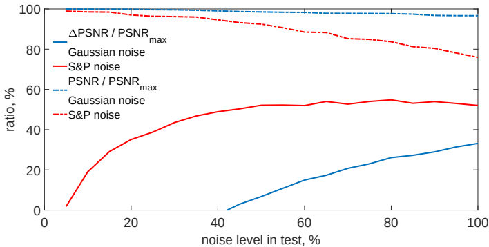
Fig. 5 The neuron-astrocyte network model robustness to noise. The dependencies of the PSNR of model recall on the noise level. The dashed lines are the PSNR of model recall related to the maximum PSNR value. The solid lines correspond to the PSNR improvement of the test image in system recall. The blue and red correspond to the Gaussian noise and salt&pepper types of noise, respectively.
