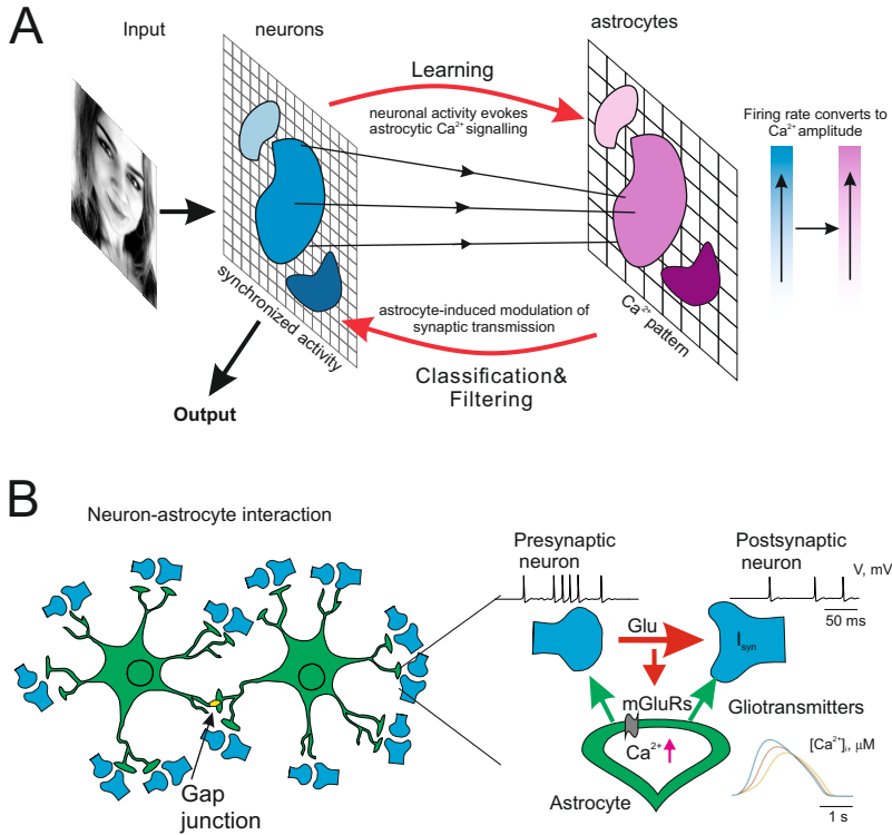
Fig. 1 (a) System concept and neuron-astrocyte network architecture. The input signal is fed to the layer of neurons. Shades of blue indicate the firing rates of corresponding neurons. Neurons and astrocytes interact bidirectionally: each astrocyte interconnected with a neuronal ensemble of N_a = 16 neurons with 4 \times 4 dimensions with overlapping in one row. Neuronal spiking rate converts to [Ca^{2+}] amplitude, in turn, astrocytes modulate synaptic transmission. The output pattern is decoded as a mean neuronal firing rate. (b) Neuron-astrocyte interaction. The synchronized activity in the neuronal ensemble triggers the elevation of intracellular Ca^{2+} concentration in astrocytes. The global events of Ca^{2+} elevation in astrocytes result in glutamate release, which can modulate the synaptic strength of all synapses corresponding to the morphological territory of a given astrocyte. We consider that the astrocytic glutamate-induced potentiation of the synapse consists in NMDAR-dependent postsynaptic slow inward currents (SICs) generation [24, 54] and mGluR-dependent heterosynaptic facilitation of presynaptic glutamate release [55–57].
