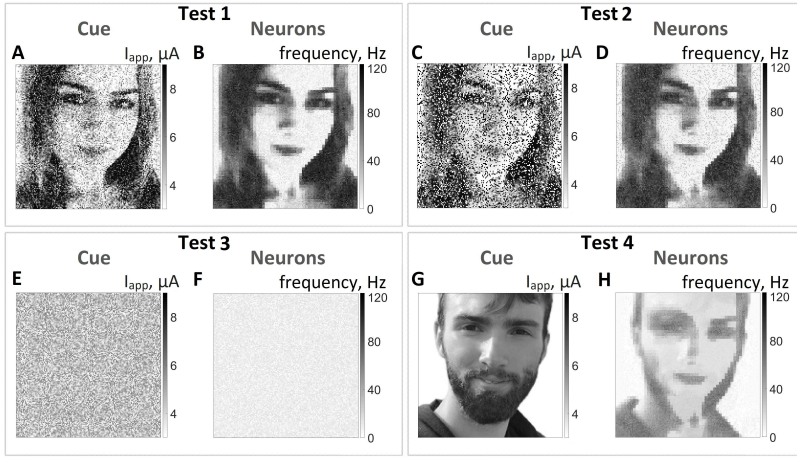
Fig. 4 Snapshots of testing neuron-astrocyte network. (a,c,e,g) are the testing input signals. (a) is the sample image distorted by 80% Gaussian noise; (c) is the sample image distorted by 40% “salt and pepper” noise; (e) uniform noise; (g) a new image. (b,d,f,h) are the neural network cued recalls. The mean neuronal firing rate in a time window of 500 ms from the beginning of the test image presentation is shown.
