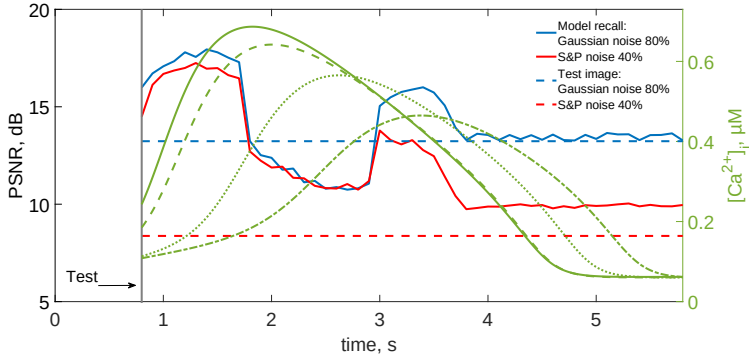
Fig. 6 The PSNR of model recall and corresponding astrocytic activity in time. The time corresponds to the moments when the test image was presented. The blue and red curves correspond to the PSNRs of the model recalls in response to test images distorted by 80% Gaussian noise and by 40 % salt&pepper noise, respectively. Examples of calcium activity in astrocytes are shown in green. The dashed lines are the PSNR of test images.
