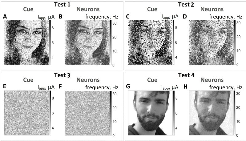
Fig. 3 Snapshots of testing the neuron-astrocyte network without modulation of synaptic transmission by astrocytes. (a,c,e,g) are the testing images. (a) is the sample image distorted by 80% Gaussian noise; (c) is the sample image distorted by 40% “salt and pepper” noise; (e) uniform noise; (g) a new image. (b,d,f,h) are the neural network cued recalls. The mean neuronal firing rate in a time window of 500 ms from the beginning of the test image presentation is shown.
