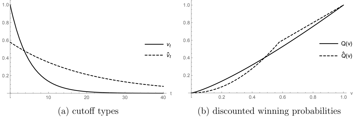
Figure 1: Improving profits through mean preserving spreads in trading times. (Parameters: (v_0, a) = (1, 4r) , (\hat{v}_0, \hat{a}) = (.577, r) , r = 0.05 .)
