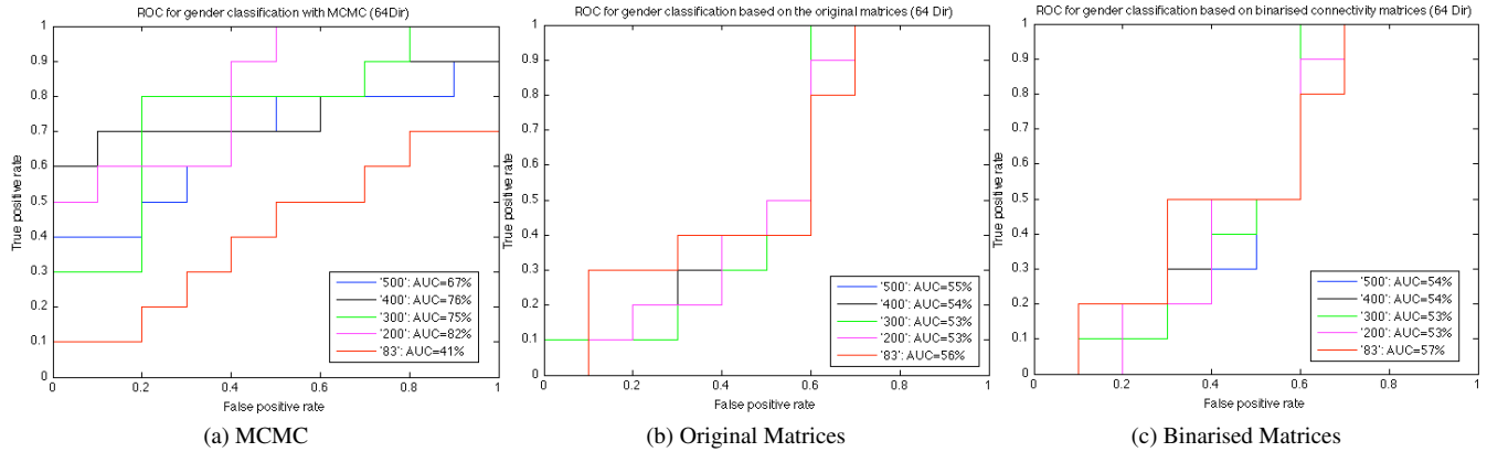
Fig. 3: ROC curves for gender classification.
