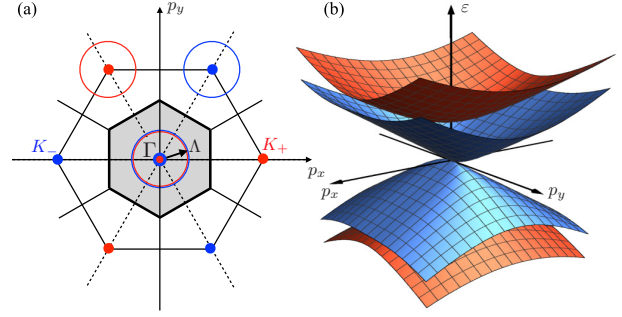
FIG. 2. (a) Gray area: folded Brillouin zone in the CDW 3 state. Valleys in the normal state (red and blue dots) fold into the center of the zone. (b) Low-energy bands of the CDW 3 state around the \Gamma point. At half-filling, the system is gapless, with semi-Dirac quasiparticles.
