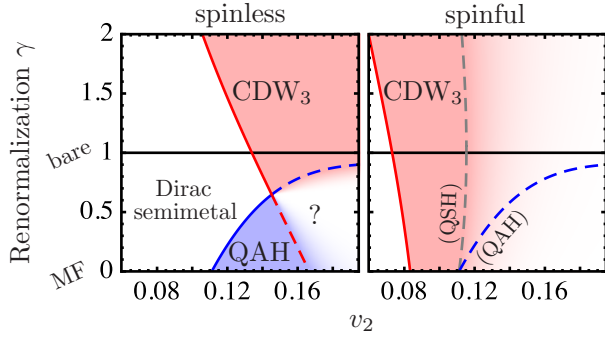
FIG. 3. Lines of critical instability along the v_2 = \frac{\pi\Lambda}{v_{FA}} V_2 axis in the presence of fluctuations, renormalized by the phenomenological parameter \gamma . The mean-field instabilities are at \gamma = 0 , the cut \gamma = 1 indicates the phase behavior without vertex renormalization. While the critical interaction strengths depend on the momentum cutoff \Lambda , the order of instabilities does not. In the regime where the NN interactions are zero ( V_1 = 0 ), the CDW_3 phases are gapless ( \Delta = 0 ).
